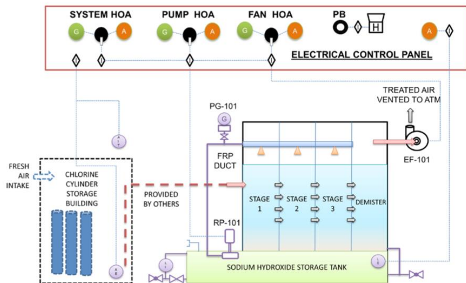
EVS-150 - Process & Instrumentation Diagram
