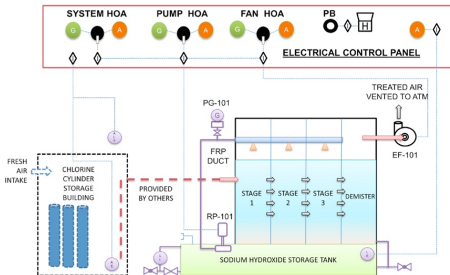
EVS-150 - Process & Instrumentation Diagram
